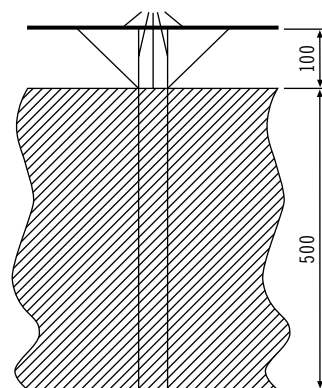
Ground pedestal
