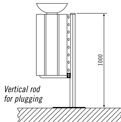
Ground pedestal
